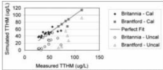
The calibrated WatPro model tracks actual measured trihalomethane concentrations more closely than the uncalibrated model.
